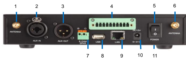
Rear panel of the Base Station, LTWI-BS750
