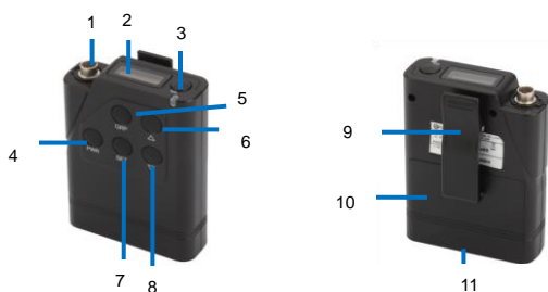
Front and rear panel of the Belt Pack, LTWI-BP750
