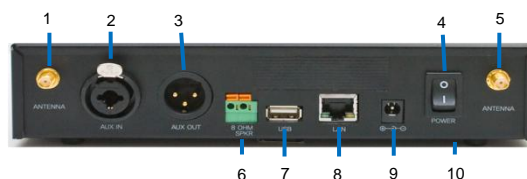
Rear panel of the Base Station, LTWI-BS250
