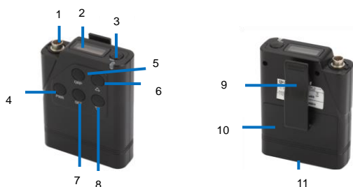
Front and rear panel of the Belt Pack, LTWI-BP250
